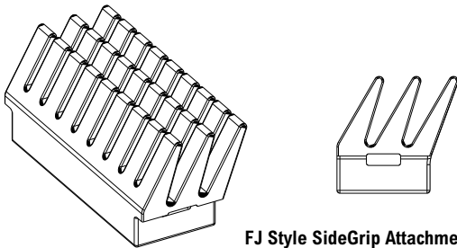
FJ Style SideGrip Attachment for any 1873 SideGrip Chain Assembly
