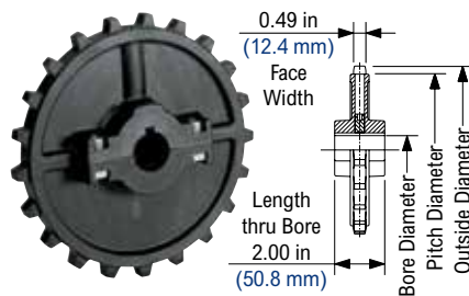
NS7700 Thermoplastic Split Sprocket
