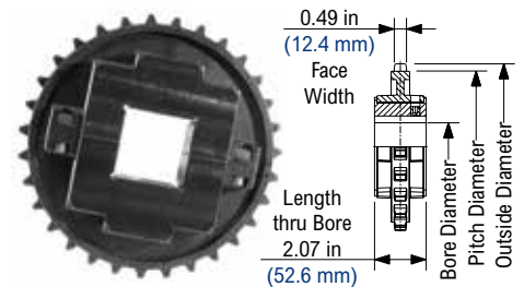
NS7700 Thermoplastic Split Sprocket with Adapter
