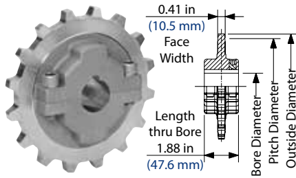
SSS7700 Stainless Steel Split Sprocket
