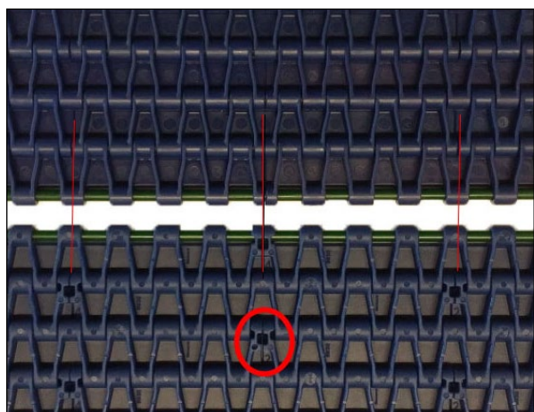
Red Encircled is the Position on the End of the Module with the Rod Retentions that Makes it Impossible to Place a Sprocket on this Position
