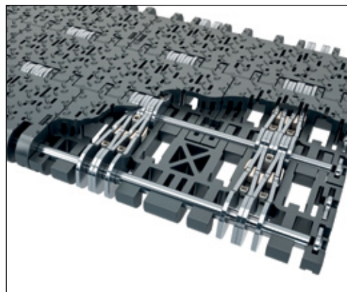
Rexnord 3122 Hybrid MatTop Chain
