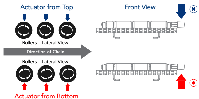
Typical Activation of ART Dynamic Chain
