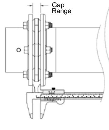
Figure 8 - Check angular alignment with Rexnord dial indicator method.
