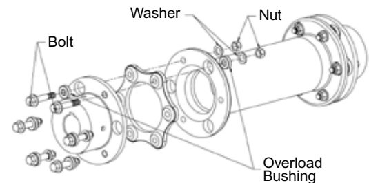
Figure 5 - Coupling assembly
