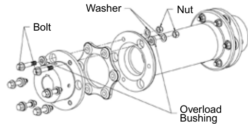
Figure 1 - Coupling assembly
