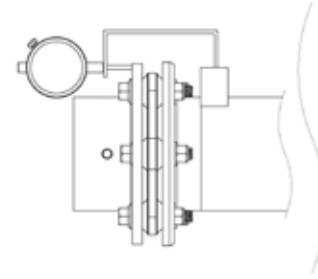
Figure 6 - Check angular alignment using dial indicator method.
