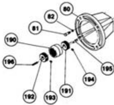
Quill Motor Flange Drive †
