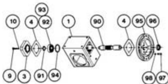
Quill Motor Flange Drive †
