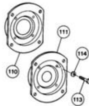
Flanged Output Drive †
