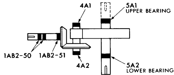
DOUBLE REDUCTION
