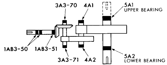
TRIPLE REDUCTION
