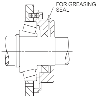
Typical High Speed Shaft
