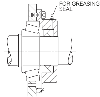
Typical High Speed Shaft
