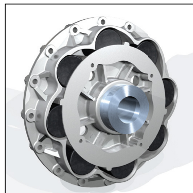
CENTAFLEX-R progressive roller coupling T = 0,25 - 15 kNm
