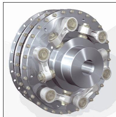
CENTAX-L for substantial misalignment T = 2 - 90 kNm
