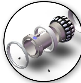
Adapter Mount
